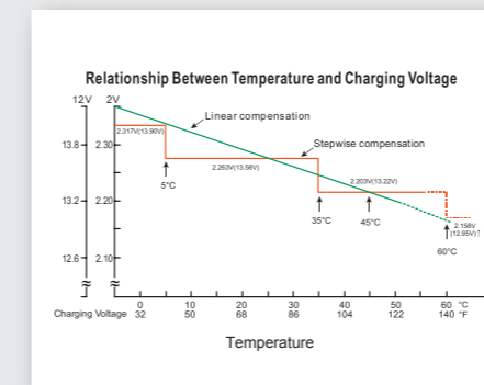
Relationship Between Temp. and Charging Voltage
