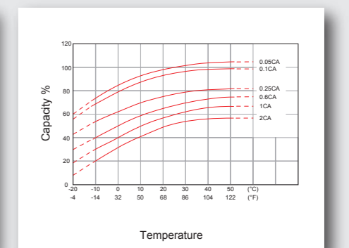
Effect of Temperature on Capacity 25°C (77°F)
